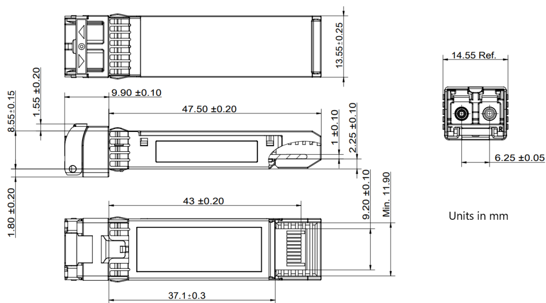
Figure2. Mechanical Outline
