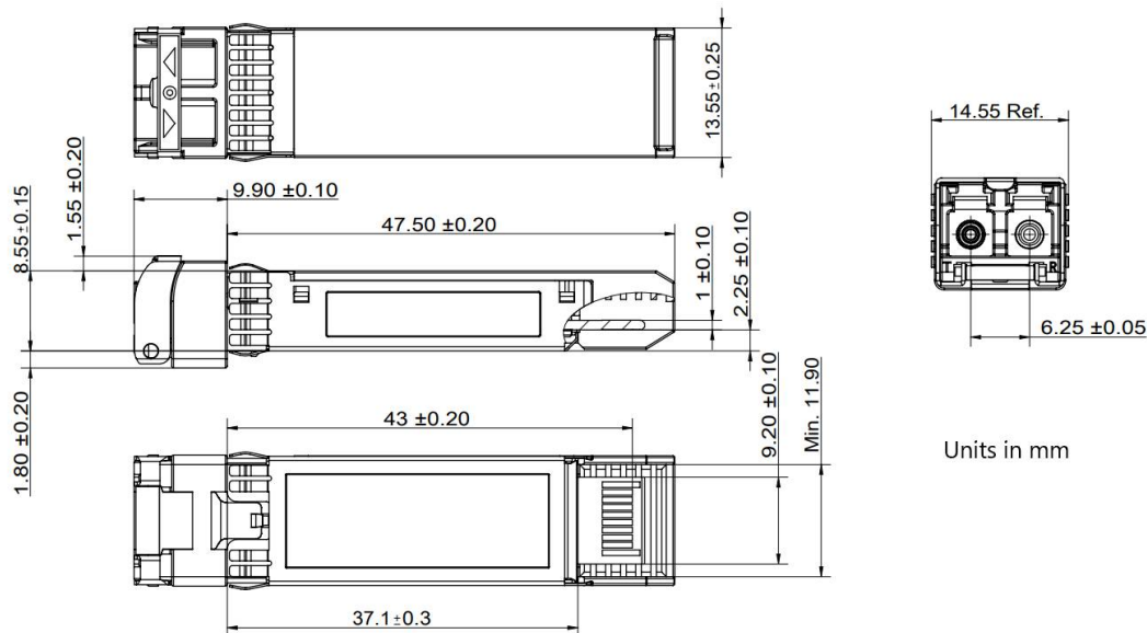
Figure2. Mechanical Outline
