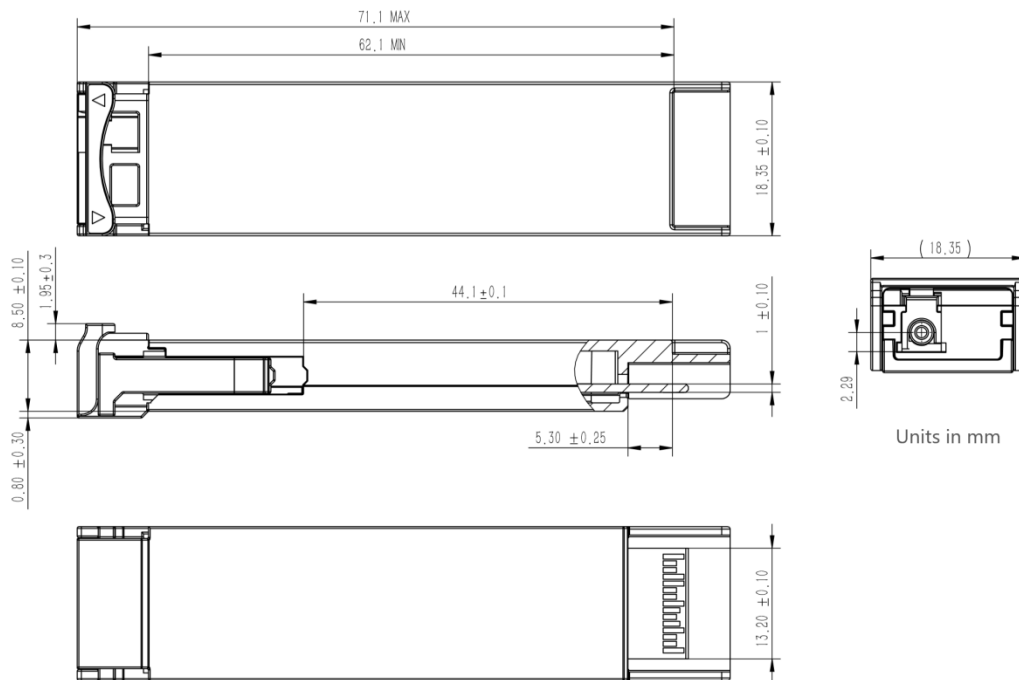
Figure2. Mechanical Outline
