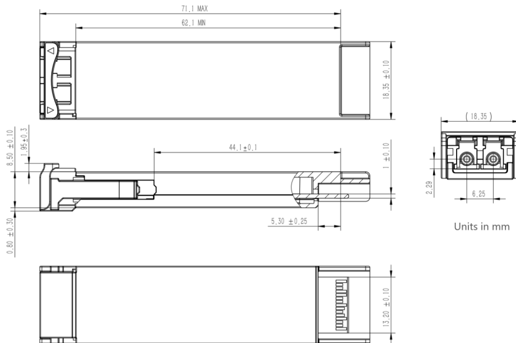
Figure2. Mechanical Outline
