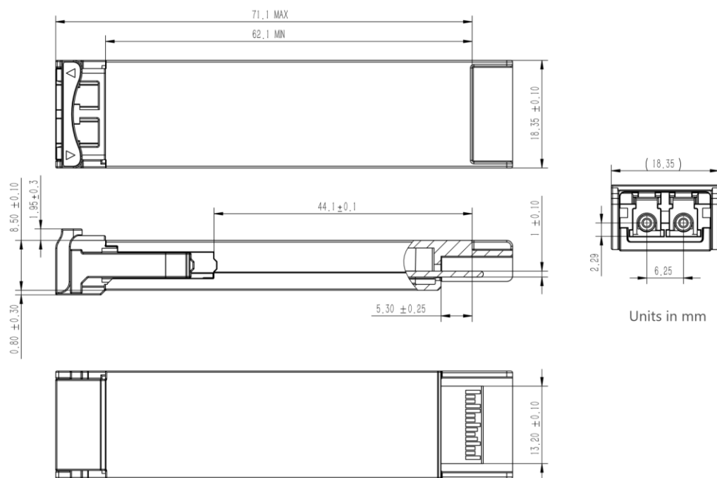
Figure2. Mechanical Outline
