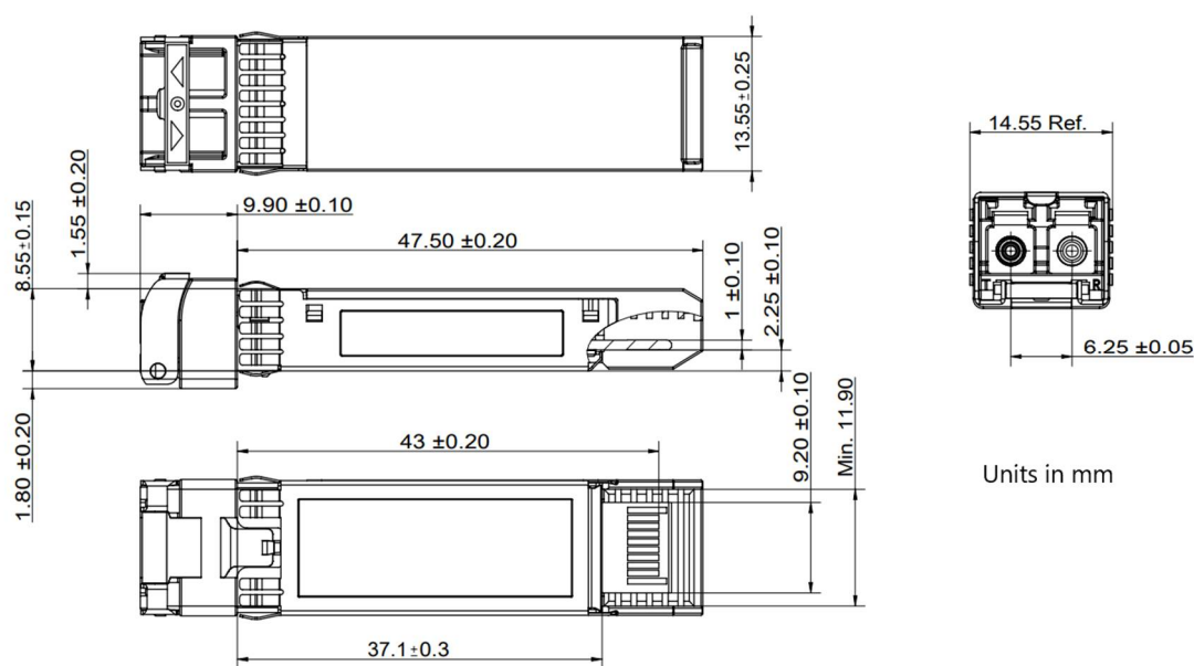
Figure2. Mechanical Outline
