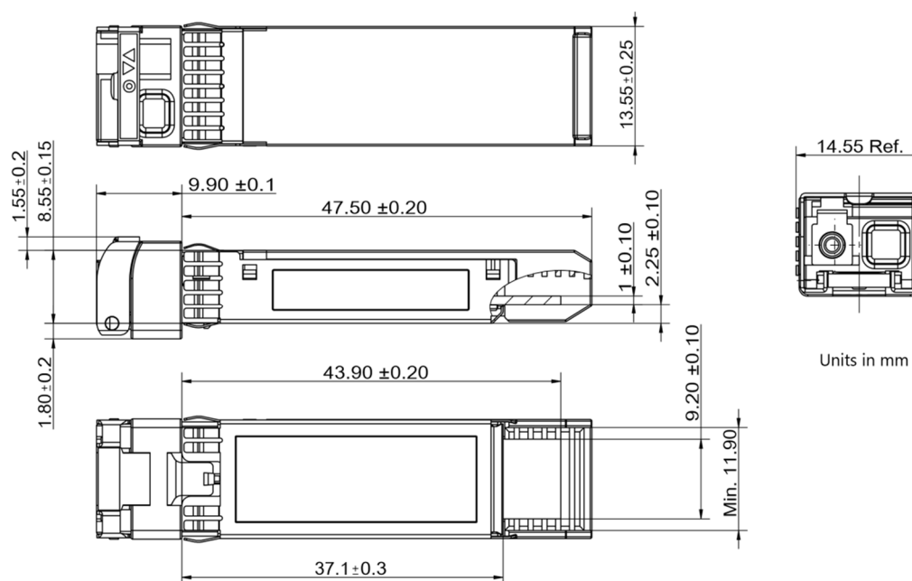
Figure2. Mechanical Outline
